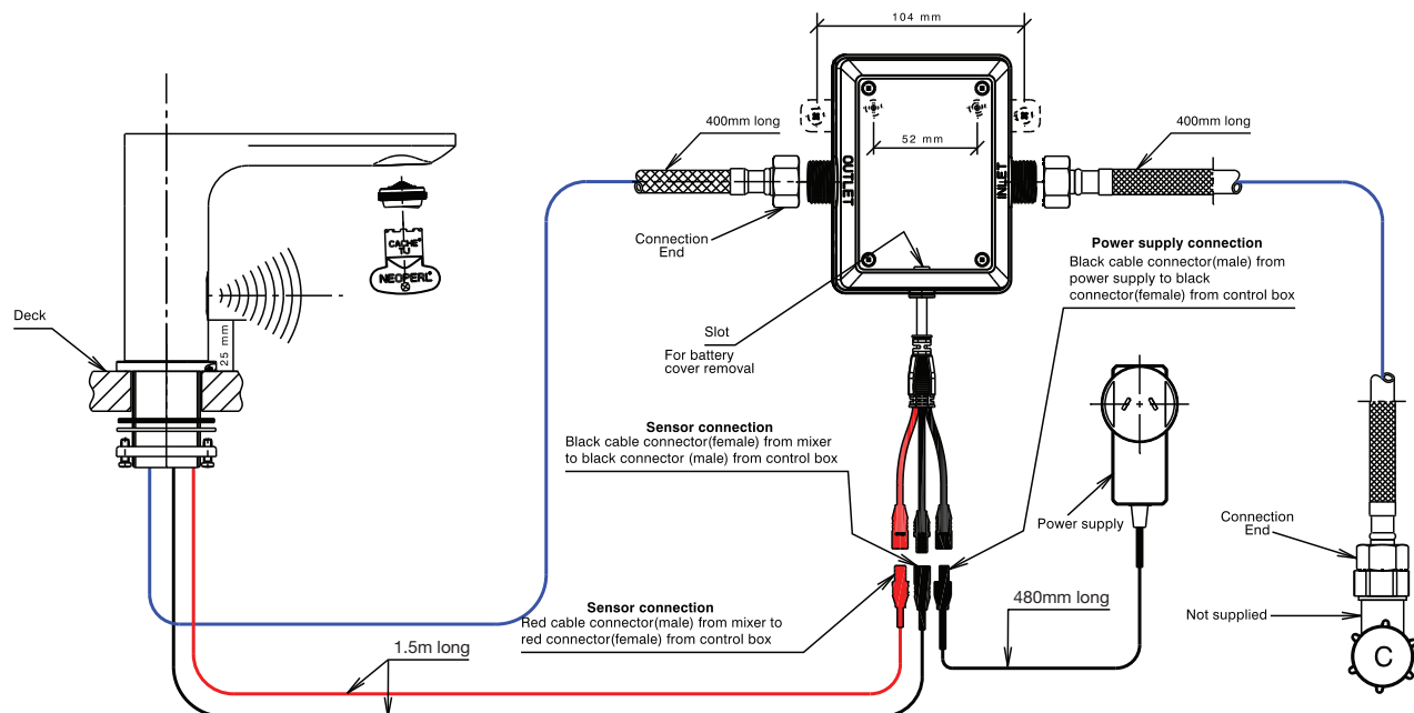
Figure 2: Sensor Activated 'Cold' Water Installation
